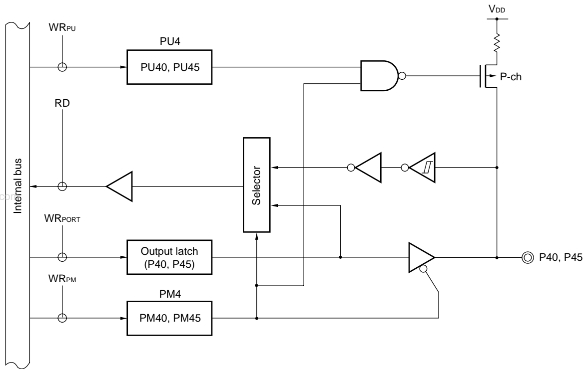
Figure 4-5. Block Diagram of P40 and P45
