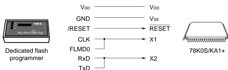
Figure 18-4. Communication with Dedicated Flash Programmer
