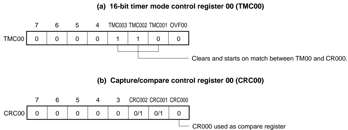
Figure 6-27. Control Register Settings in Square-Wave Output Mode (1/2)
