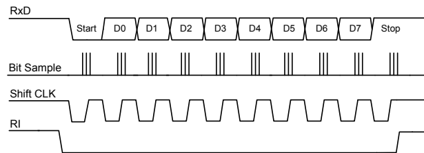
Receive Timing of Mode 1
