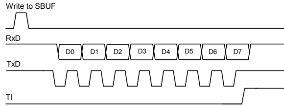
Send Timing of Mode 0
