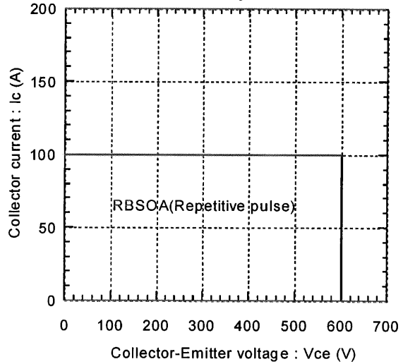
Reversed biased safe operating area Vcc=15V, Tj≤125°C
