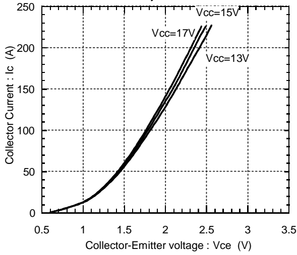
Collector current vs. Collector-Emmitter voltage T_j=25^{\circ}\text{C}
