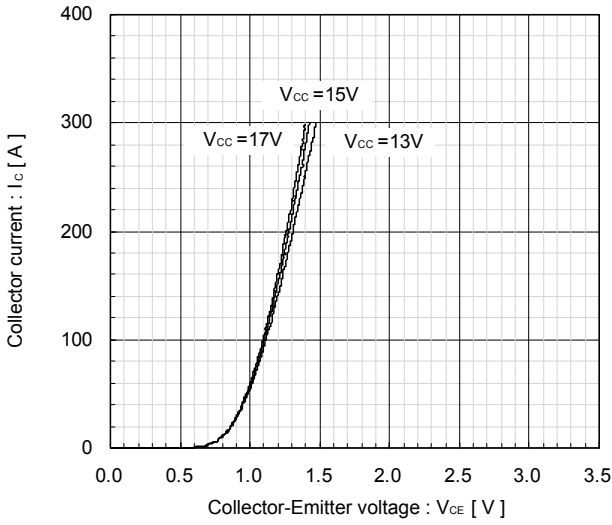
Collector current vs. Collector-Emittor voltage T_j = 25^\circ\text{C} [Chip] (typ.)
