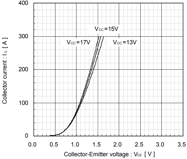
Collector current vs. Collector-Emittor voltage T_j = 125^\circ\text{C} [Chip] (typ.)
