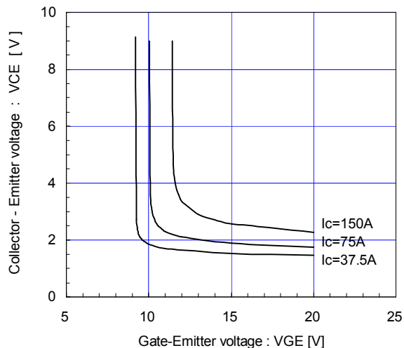
[ Inverter ] Collector-Emitter voltage vs. Gate-Emitter voltage (typ.) T j =25°C / chip
