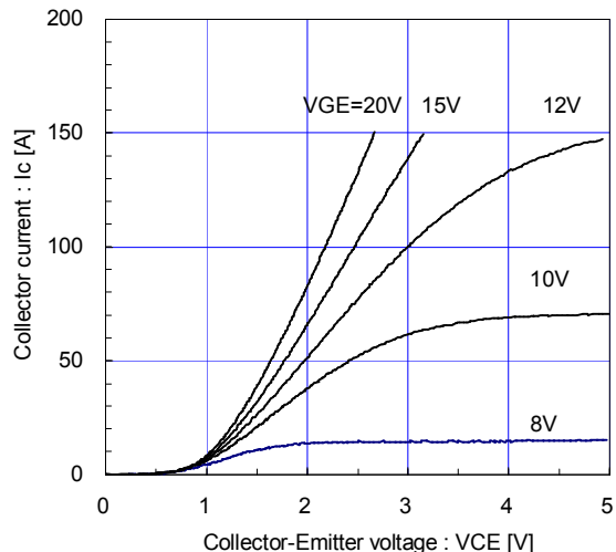
[ Inverter ] Collector current vs. Collector-Emitter voltage (typ.) T j = 125°C / chip
