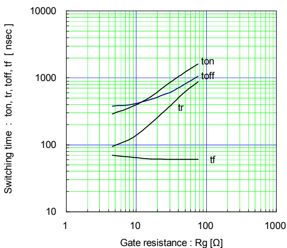
[ Inverter ] Switching time vs. Gate resistance (typ.) V_{cc}=600V, I_c=100A, V_{GE}=\pm 15V, T_j=25^\circ C
