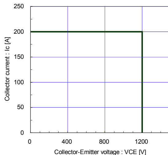
[ Inverter ] Reverse bias safe operating area (max.) +V_{GE}=15V, -V_{GE} \le 15V, R_g \ge 9.1\Omega, T_j \le 125^\circ C
