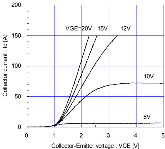
[ Inverter ] Collector current vs. Collector-Emitter voltage (typ.) T j = 25°C / chip
