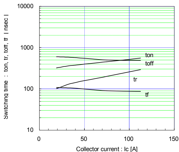
[ Inverter ] Switching time vs. Collector current (typ.) V_{cc}=600V, V_{GE}=\pm 15V, R_g=9.1\Omega, T_j=125^\circ C
