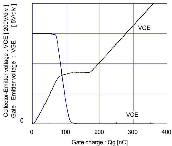
[ Inverter ] Dynamic Gate charge (typ.) Vcc=600V, Ic=100A, T j = 25°C
