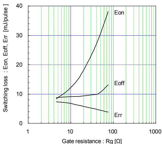
[ Inverter ] Switching loss vs. Gate resistance (typ.) V_{cc}=600V, I_c=100A, V_{GE}=\pm 15V, T_j=125^\circ C
