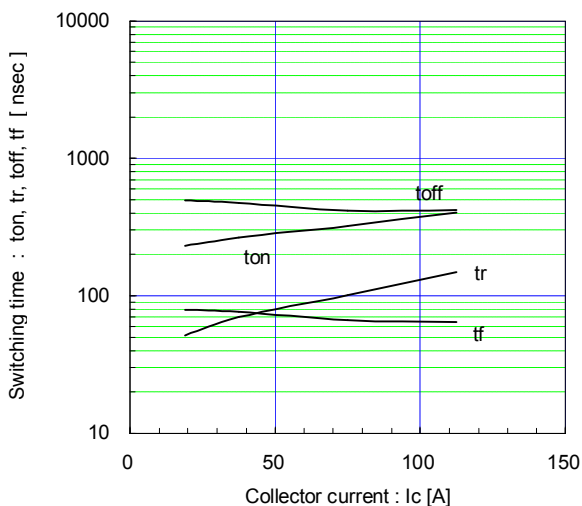
[ Inverter ] Switching time vs. Collector current (typ.) V_{cc}=600V, V_{GE}=\pm 15V, R_g=9.1\Omega, T_j=25^\circ C
