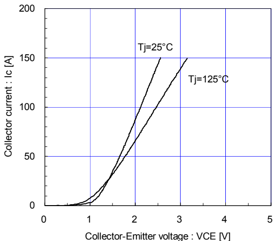
[ Inverter ] Collector current vs. Collector-Emitter voltage (typ.) VGE=15V / chip
