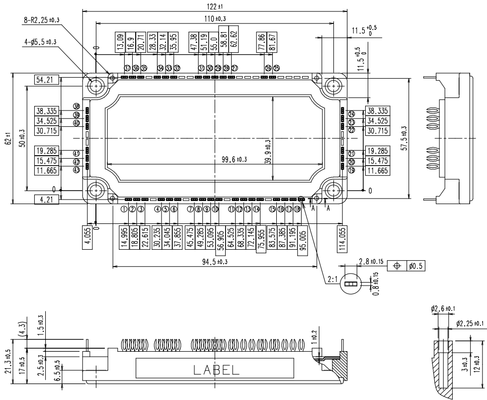
Section A-A Weight: 310g(typ.)
