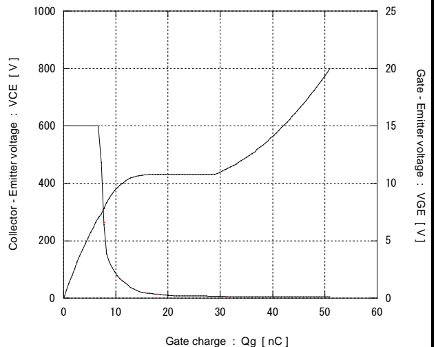
[ Inverter ] Dynamic Gate charge (typ.) Vcc = 600V, Ic = 15A, T j = 25°C
