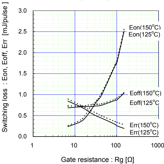
[ Inverter ]
