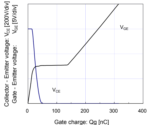
[ Inverter ] Dynamic gate charge (typ.) V_{CC} = 600\text{V} , I_c = 35\text{A} , T_j = 25^\circ\text{C}
