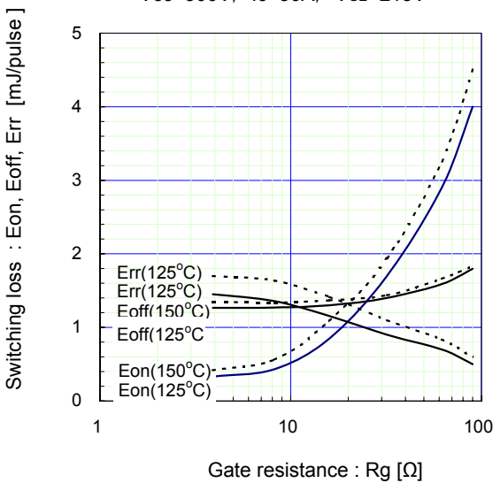
[ Inverter ]
