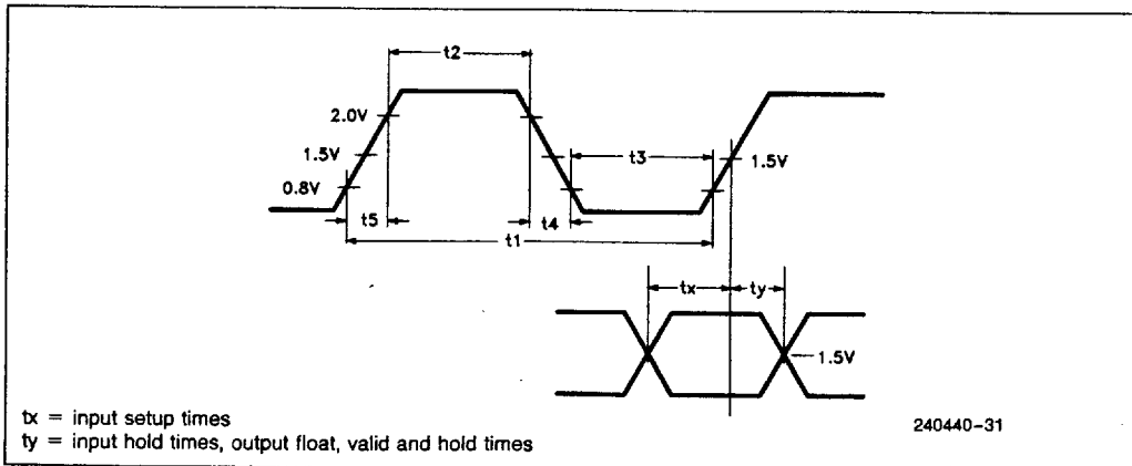
Figure 6.2. CLK waveform
