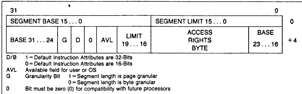
Figure 4.6. Segment Descriptors
