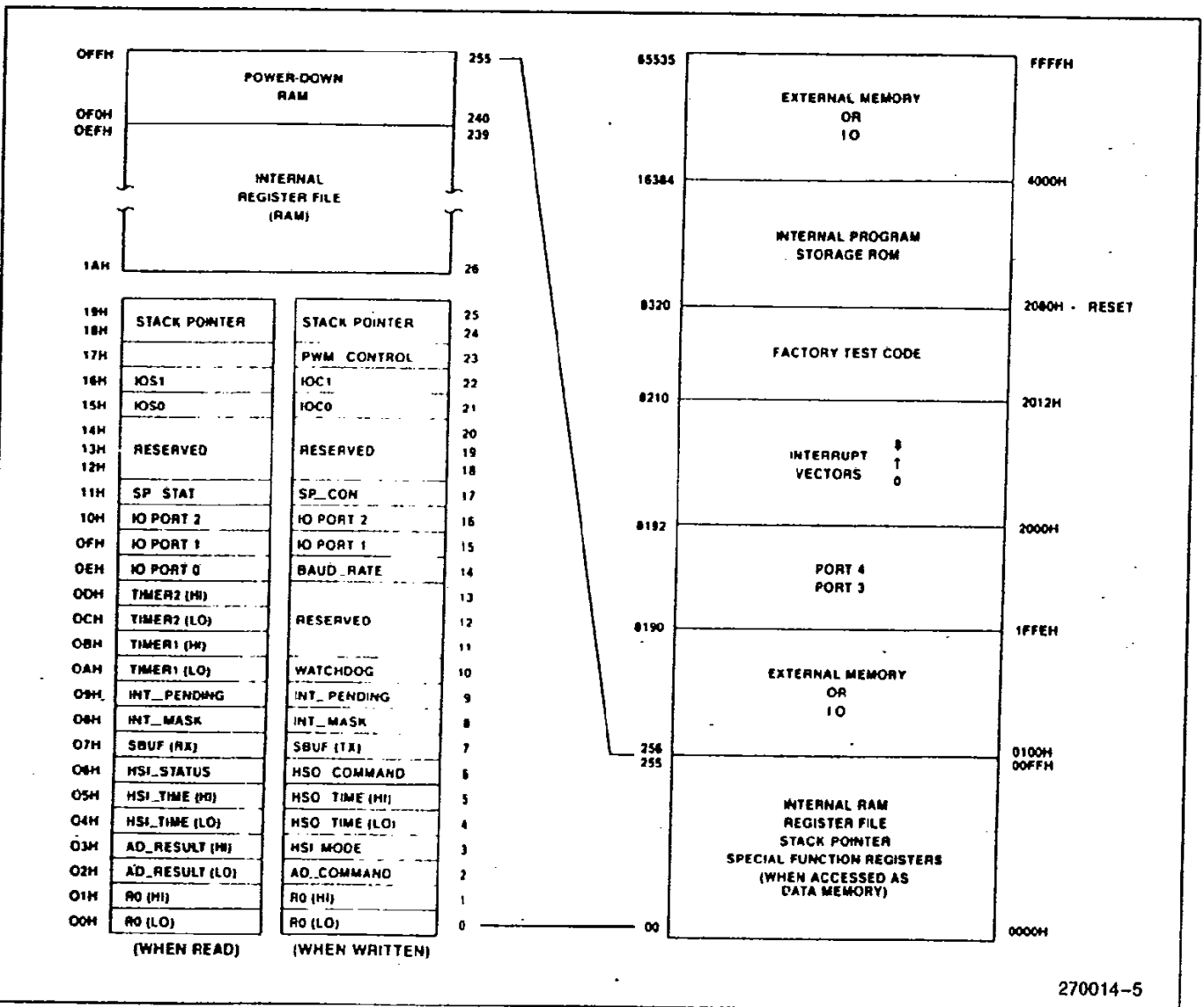
Figure 5. Memory Map
