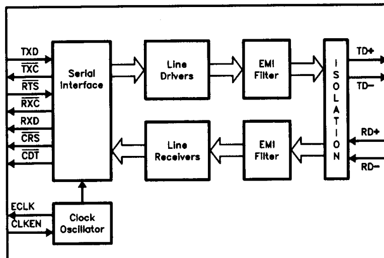
82521TA Block Diagram
