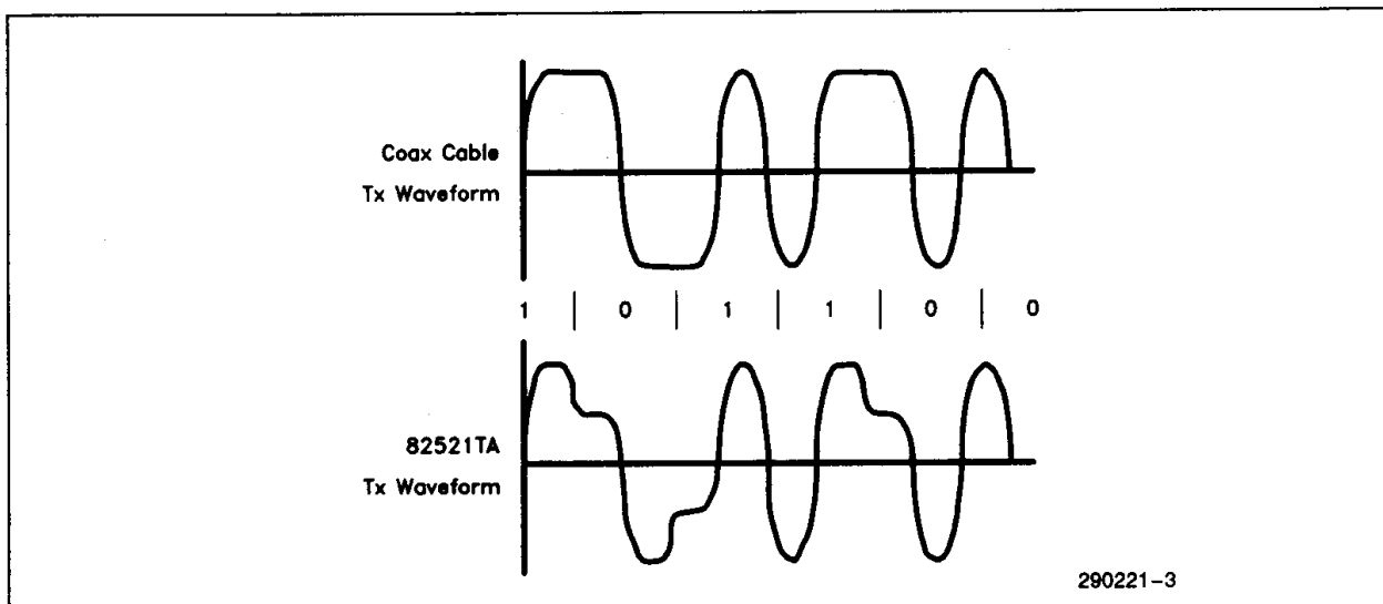
Figure 1. Effects of Predistortion
