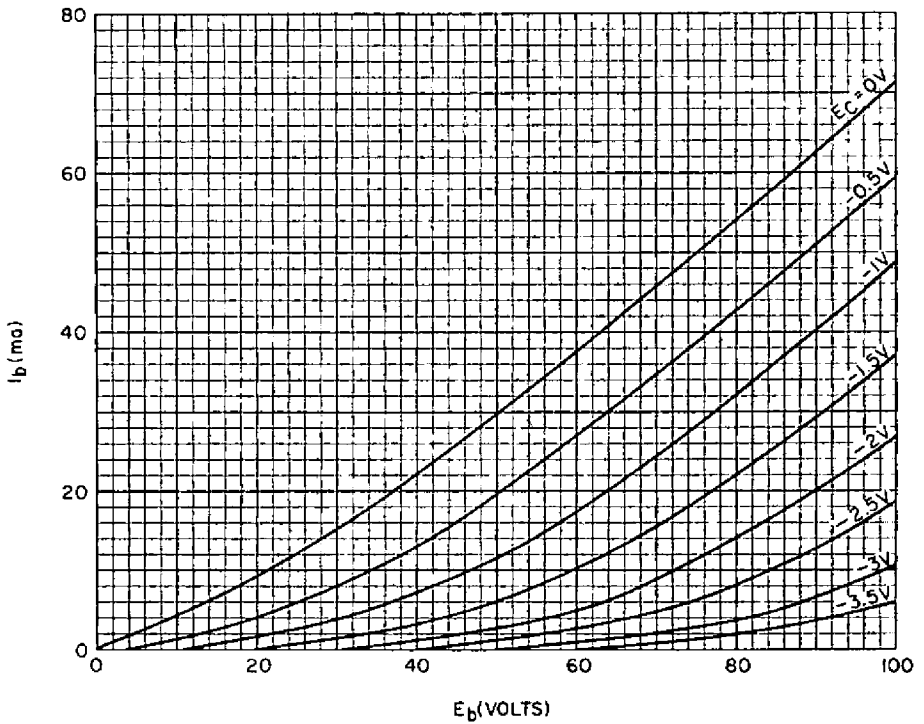
PLATE CHARACTERISTICS
