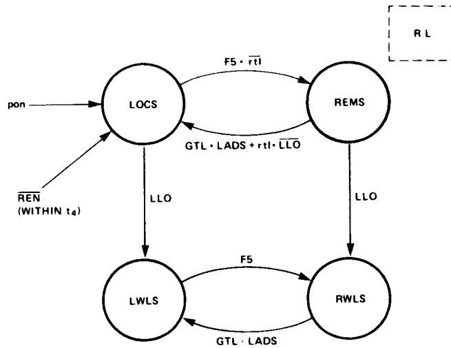
Figure A-1. 8291A State Diagrams (Continued)
