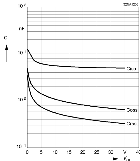
Fig. 6 Typ. capacitances vs. V_{CE}
