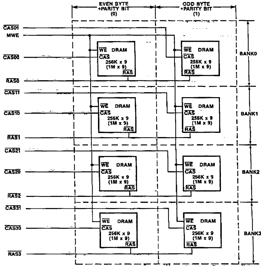
Figure 2.4 DRAM Organization
