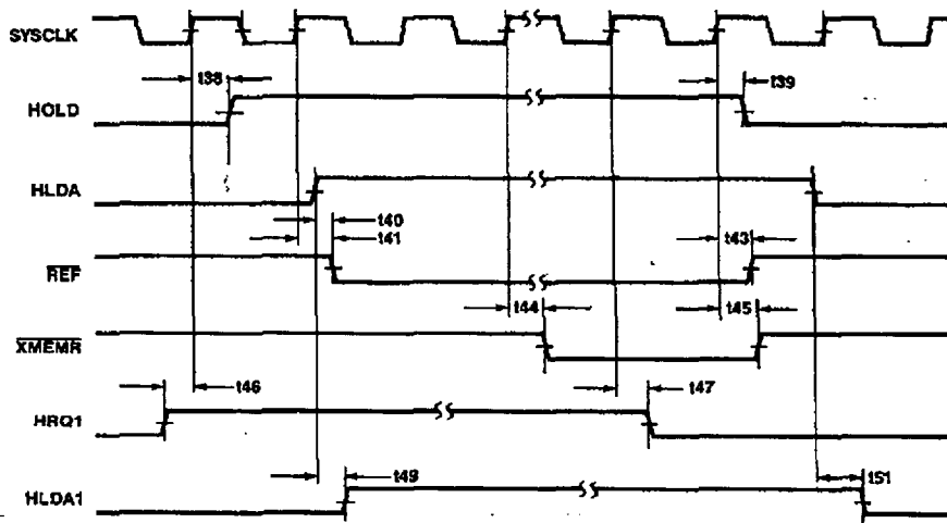
Refresh/DMA Cycle
