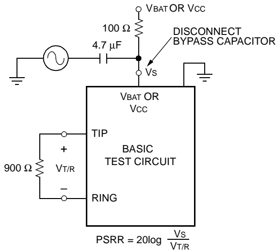
Figure 6. Metallic PSRR
