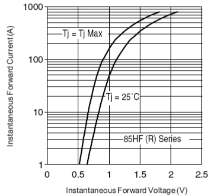
Fig. 12 - Forward Voltage Drop Characteristics (for 1400 V, 1600 V)
