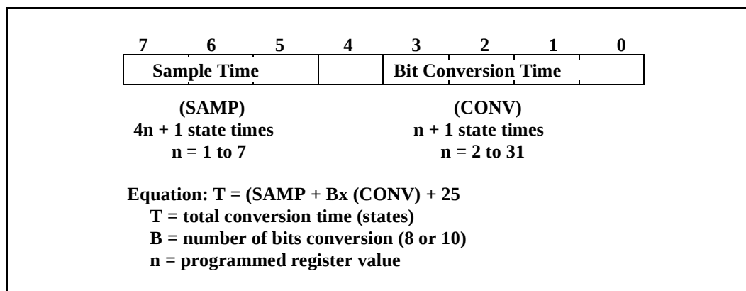
Figure 22. AD_TIME 1FAFH:Byte
