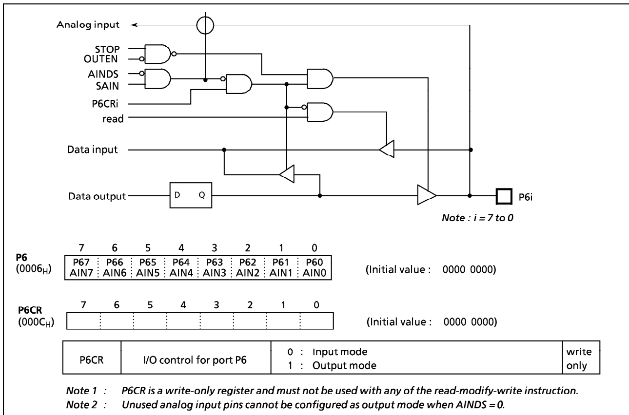
Figure 2-6. Port P6
