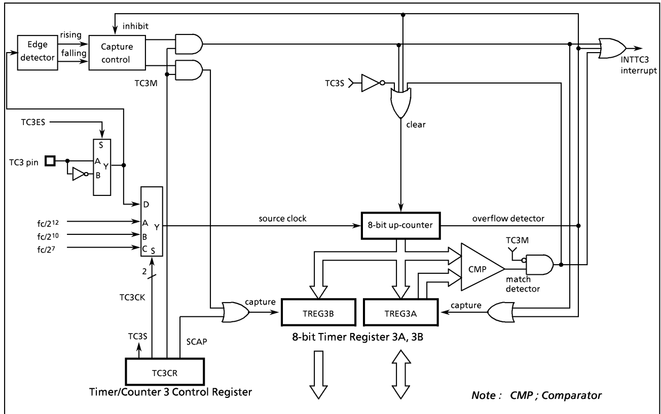
Figure 2-21. Timer/Counter (TC3)
