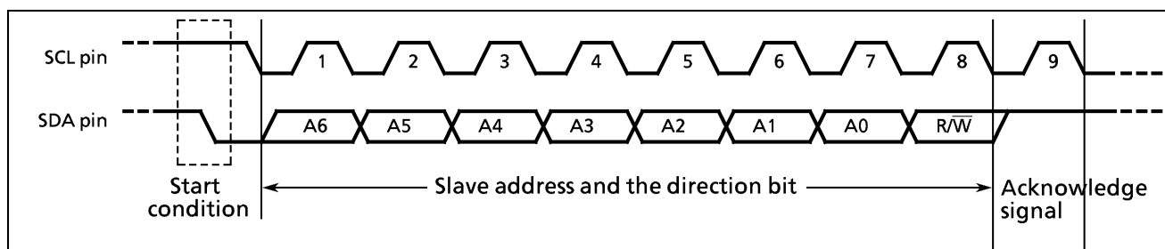
Figure 2-33. Start Condition Generation and Slave Address Generation
