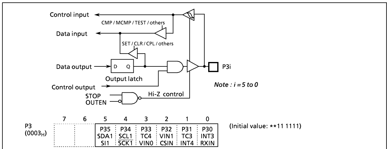
Figure 2-4. Port P3
