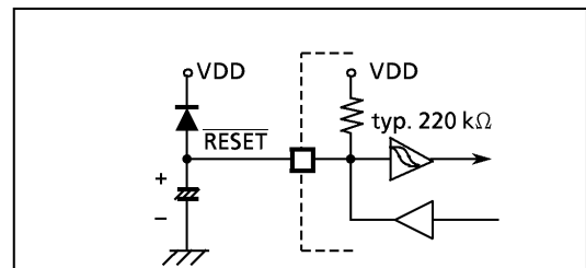
Figure 1-28. Simple Power-on-Reset Circuitry
