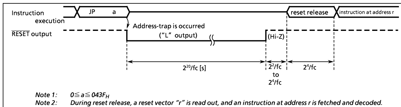
Figure 1-29. Address-Trap-Reset
