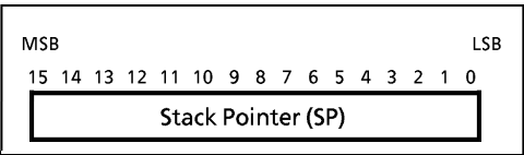
Figure 1-7. Stack Pointer
