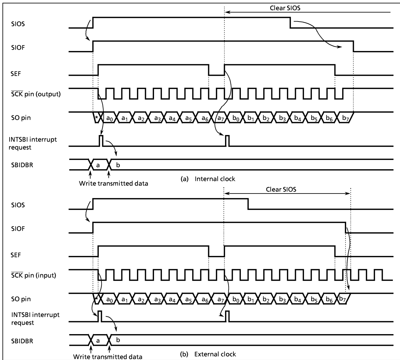
Figure 2-45. Transfer Mode
