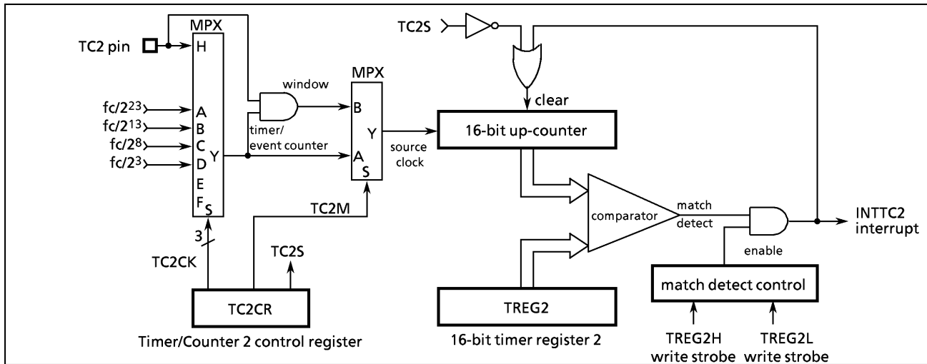
Figure 2-18. Timer/Counter 2 (TC2)
