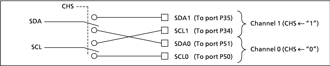
Figure 2-31. Channel Selection
