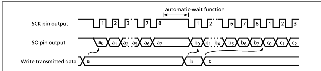
Figure 2-42. Automatic-wait Function
