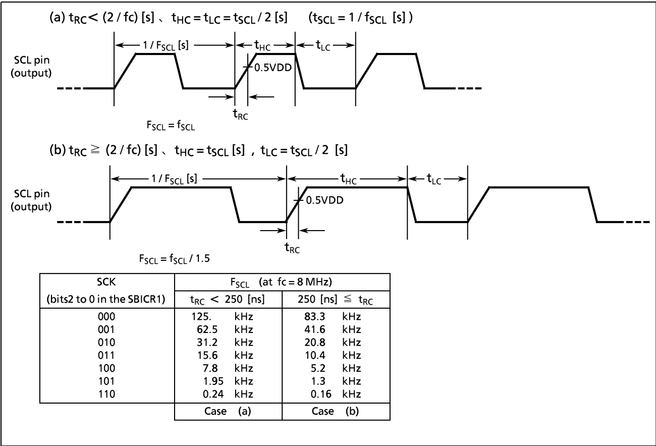
Figure 2-32. Serial Clock
