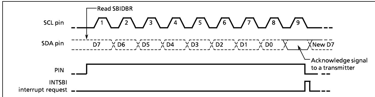
Figure 2-37. Example of Receiving Data
