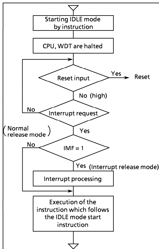
Figure 1-18. IDLE Mode
