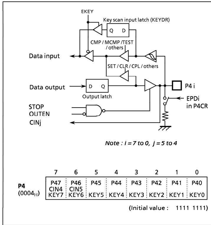
Figure 2-7. Port P4
