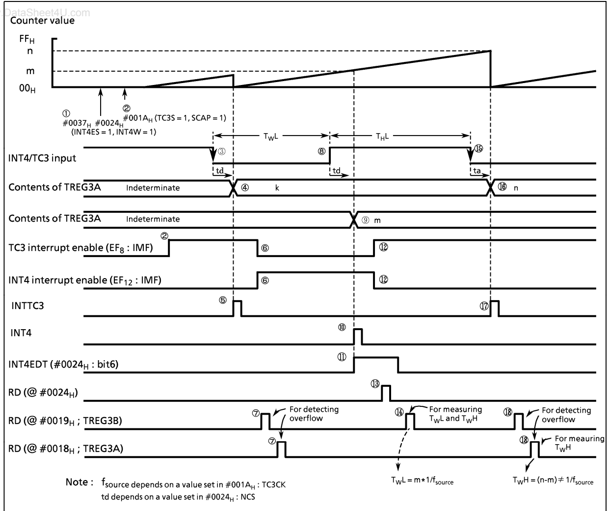
Figure 2-33. Example of remote control waveform by timer 3 (in capture mode)
