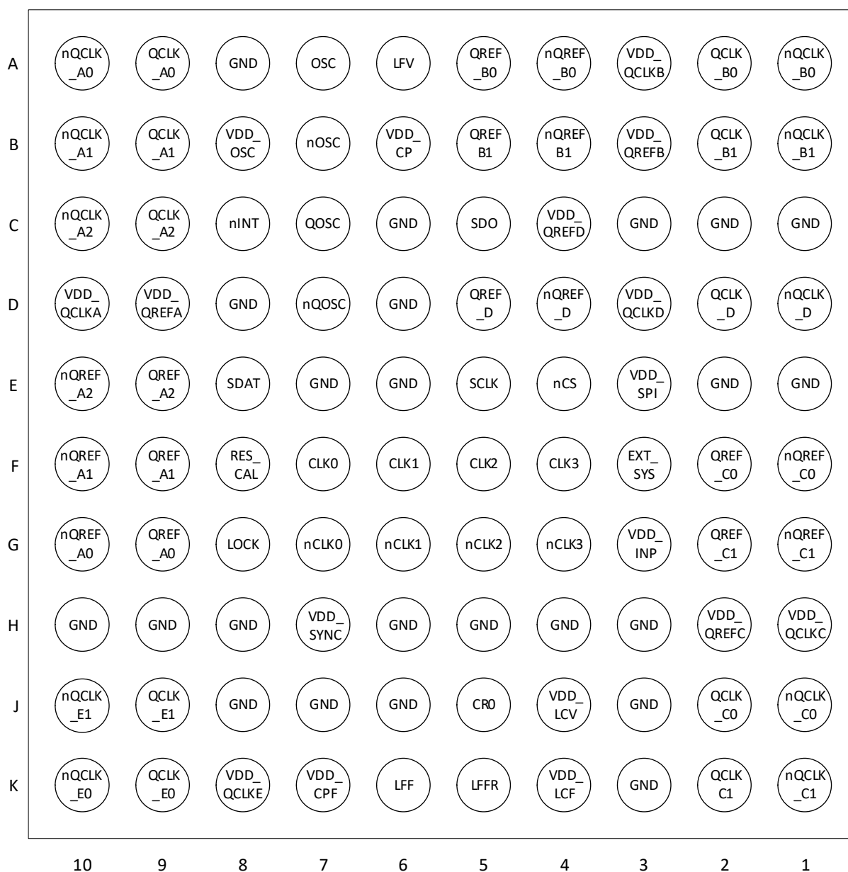
Figure 2. Ball Map for 100-CABGA, 1mm Ball Pitch 11 × 11 × 1.1 mm Package (Bottom View)
