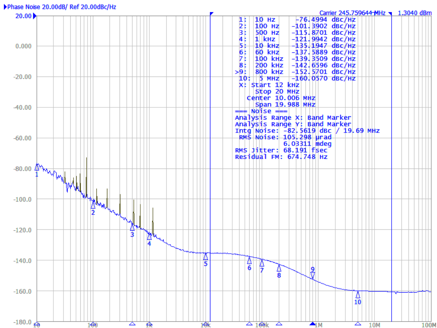
Figure 12. 245.76MHz Output Phase Noise
