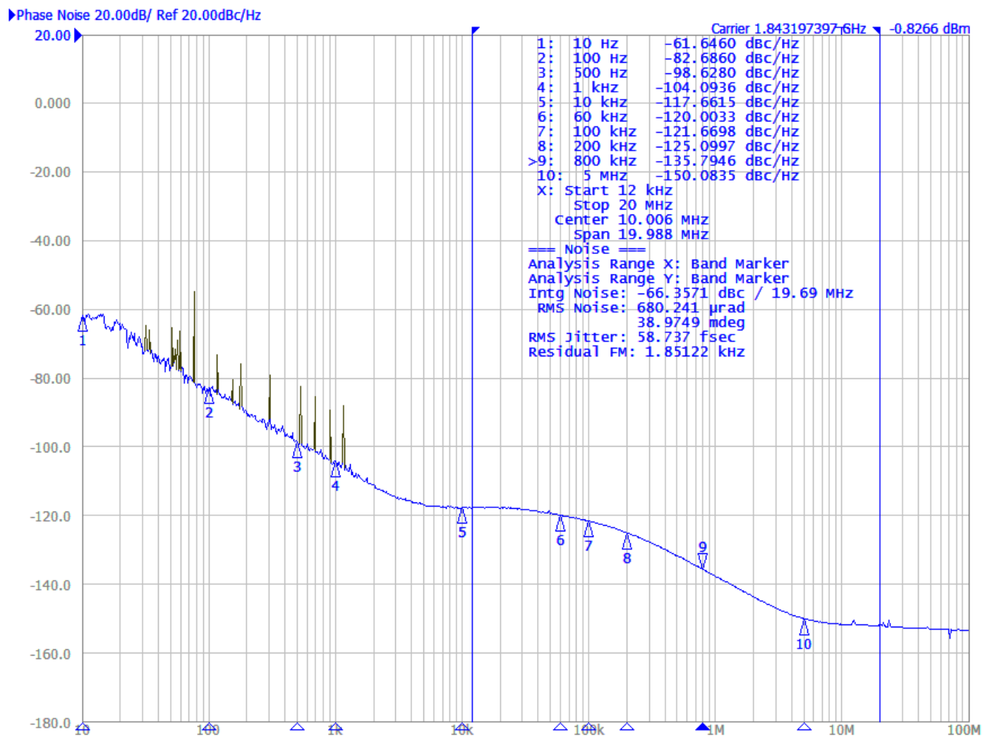
Figure 9. 1843.2MHz Output Phase Noise
