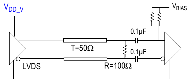
Figure 14. LVDS (STYLE = 0) AC Output Termination
