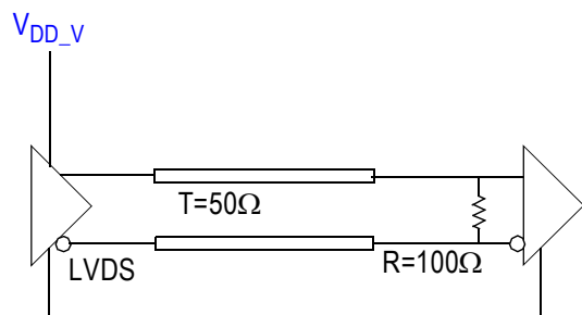
Figure 13. LVDS (STYLE = 0) Output Termination
