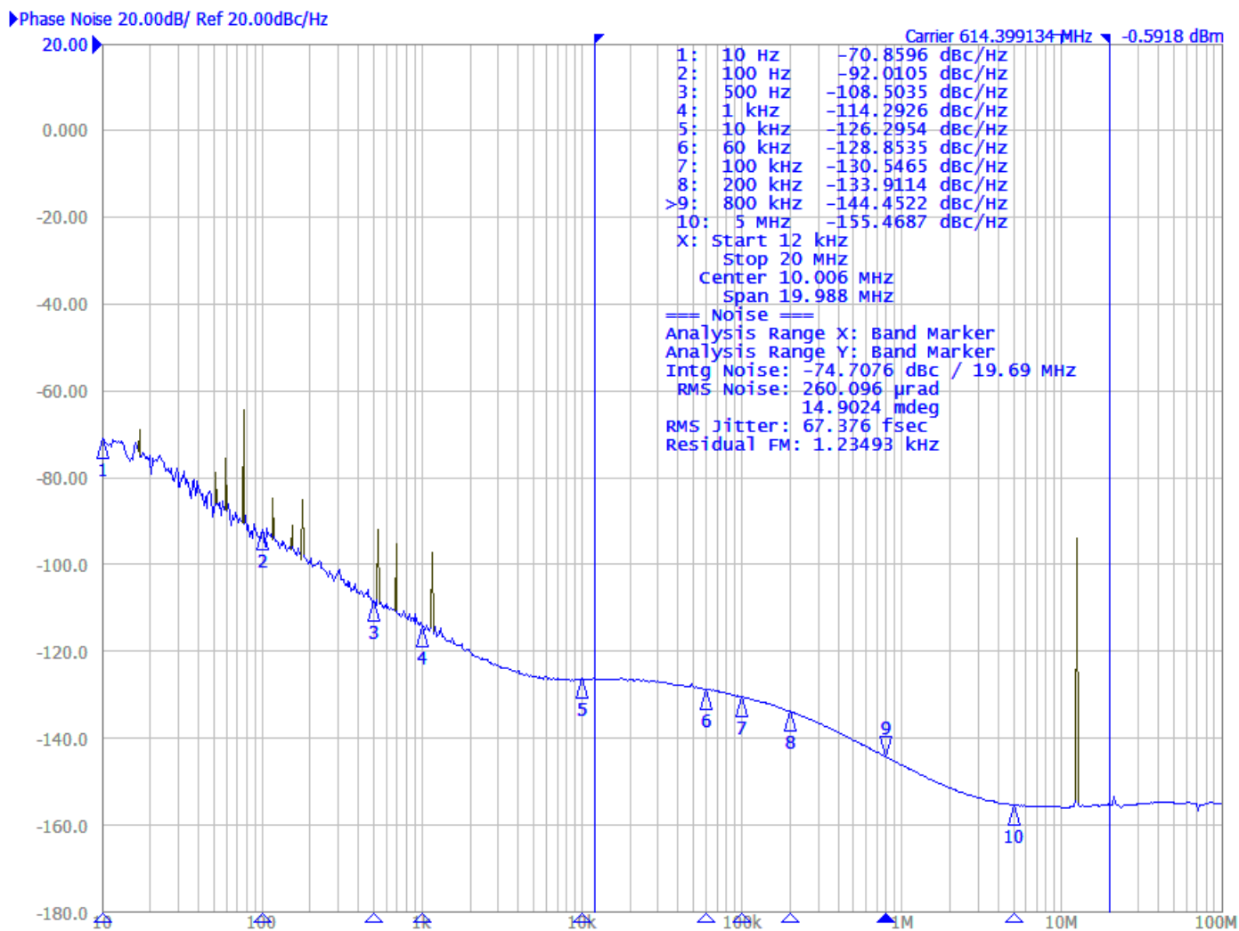
Figure 10. 614.4MHz Output Phase Noise
