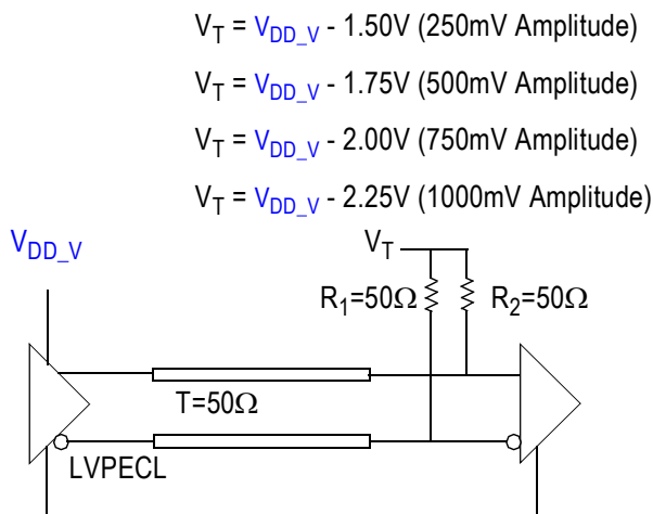
Figure 16. LVPECL (STYLE = 1) Output Termination
