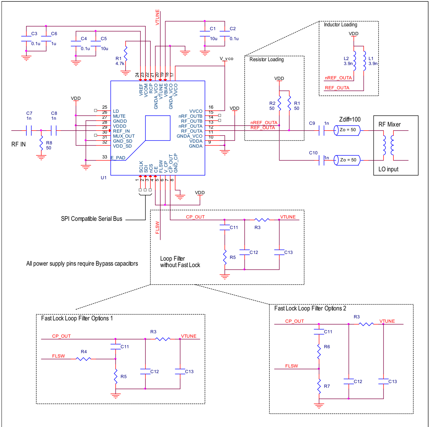
Figure 13A. 8V97051A General Application Schematic Example
