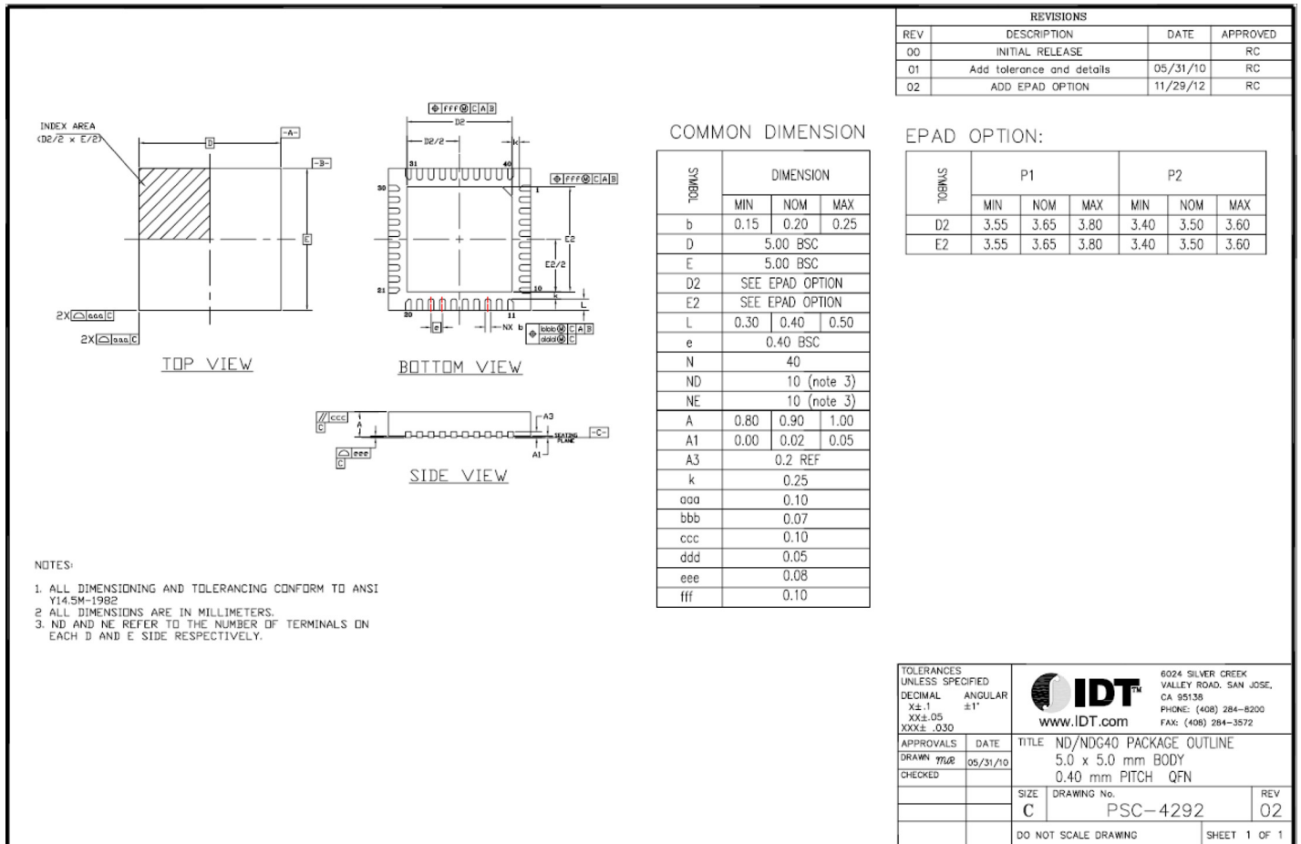
Figure 16. 40-QFN Package Diagram
