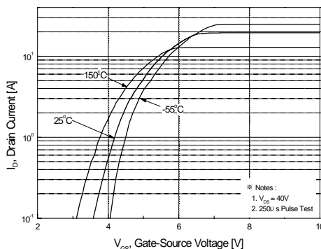
Figure 2. Transfer Characteristics
