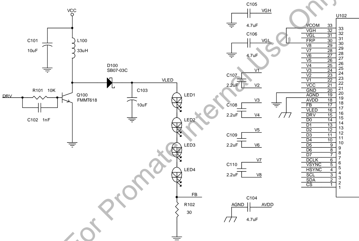
Fig.11 Typical Application Circuit
