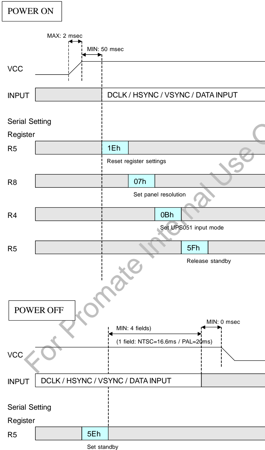
Fig 15. Recommend Serial Command Settings
