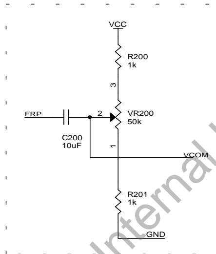
Fig.13 Optional VCOM-DC External Adjustment Circuit
