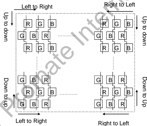
Fig. 10 Color filter arrangement for 960x240 resolution
