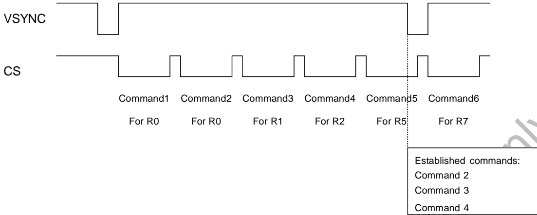
Fig. 6 Illustration of Serial Command Operation
