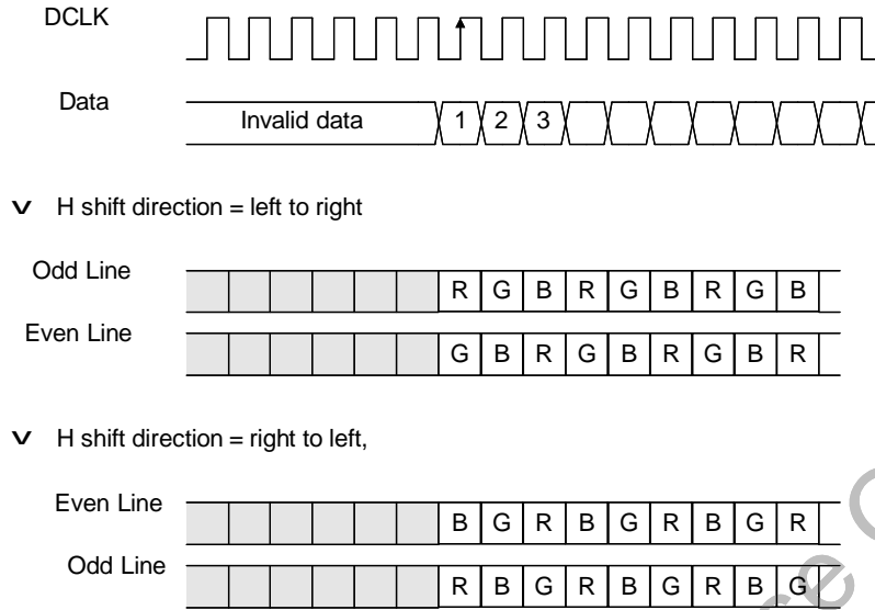
Fig. 9 UPS051 Input RGB sequence for 960x240 resolution
