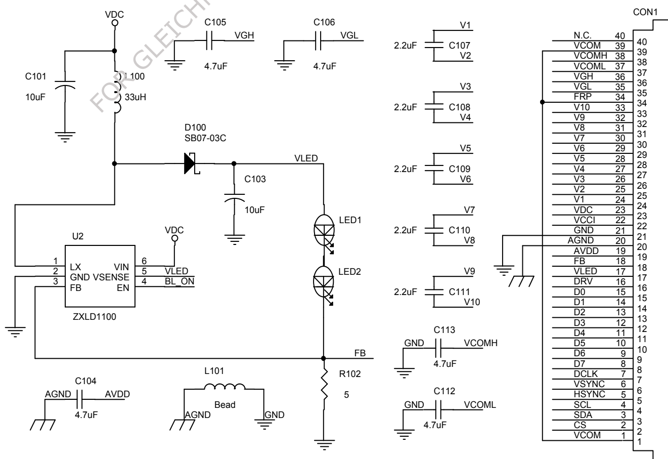
Fig.13 External LED driver Circuit
