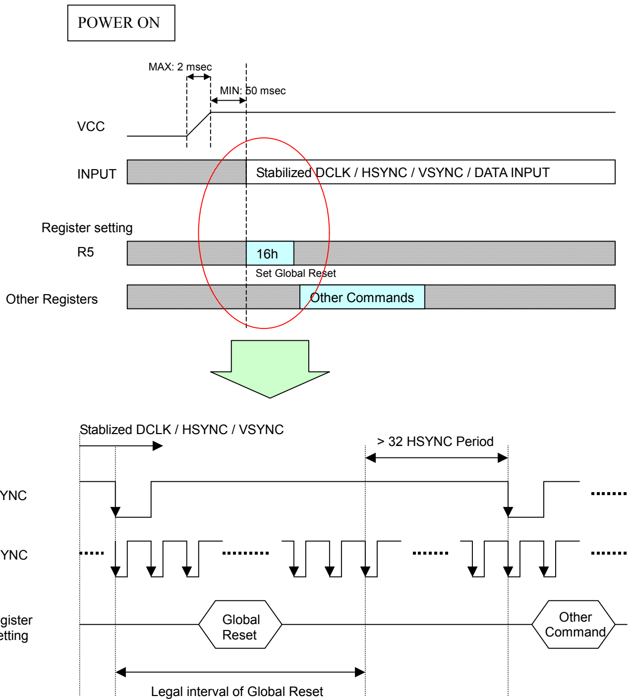
Fig.19 Valid Timing of Global Reset
