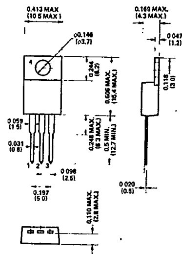
1: Base 2: Collector 3: Emitter 4: Fin (Collector) Dimension in inches and (millimeters)
