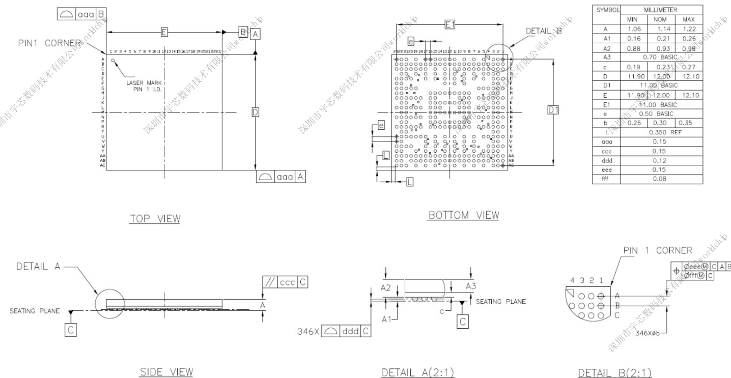
Figure 7-2. A133 Package Dimension
