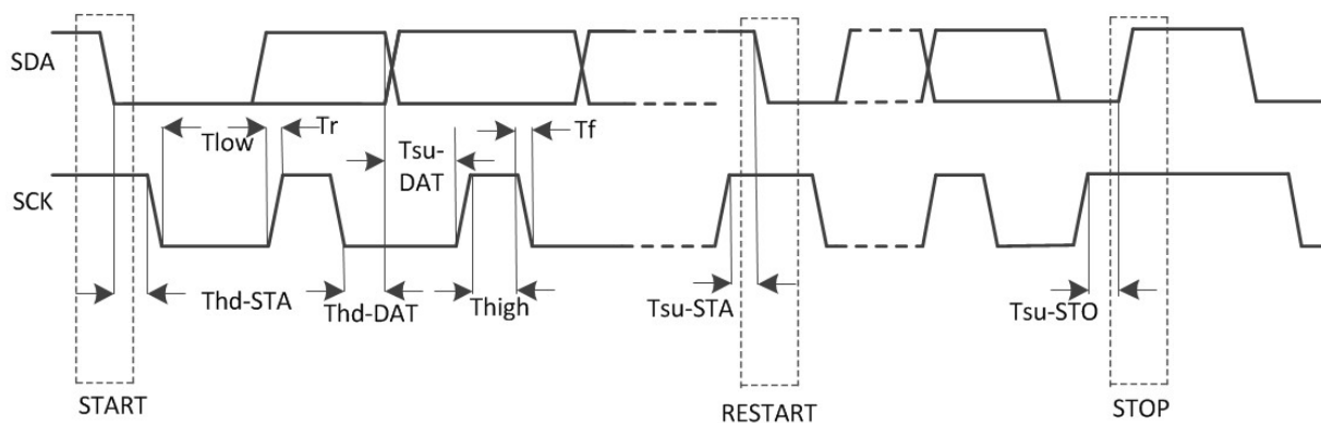
Figure 5-50. TWI Timing
