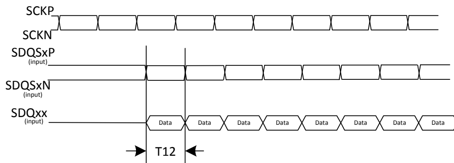
Figure 5-7. LPDDR3 Read Cycle
