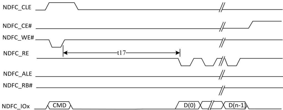
Figure 5-21. WE# High to RE# Low Timing
