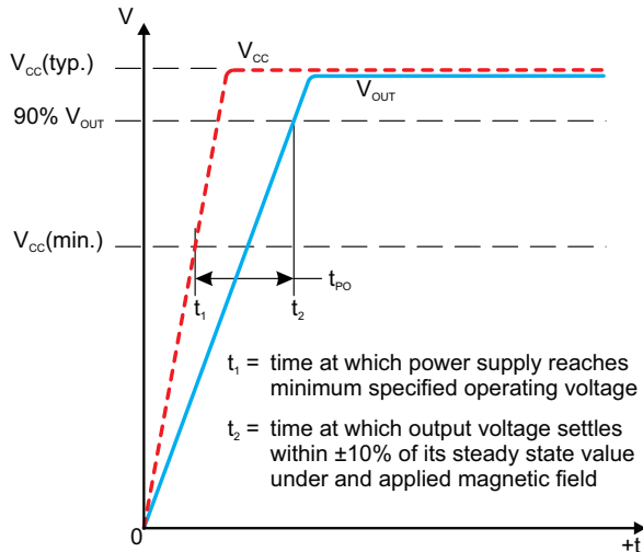
Figure 1: Power-On Time
