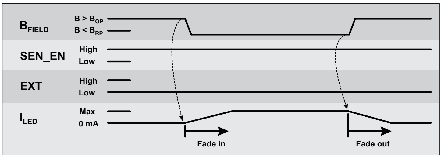
Figure 3: Hall-Activated Operation
