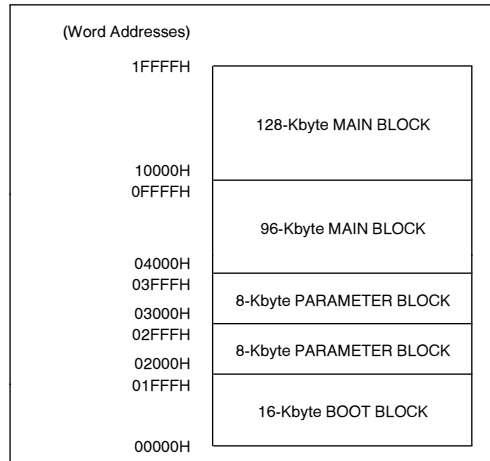
Figure 4. A28F200BX-B Memory Map
