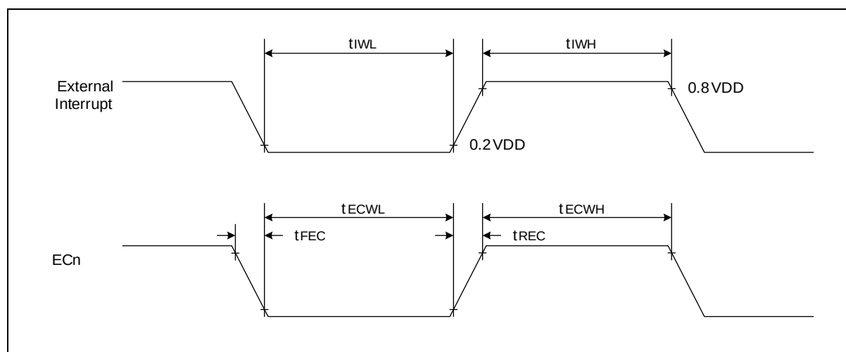
Figure 47. Timing Diagram of External Input AC Characteristics Definitions
