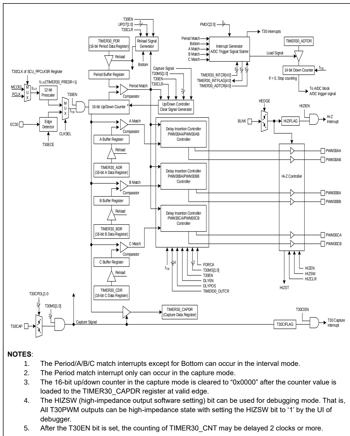
Figure 31. Timer Counter 30 Block Diagram
