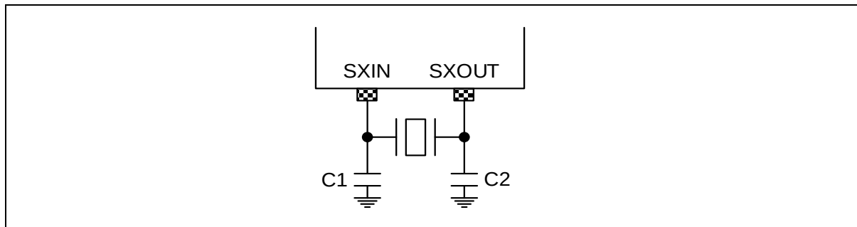
Figure 45. Crystal Oscillator
