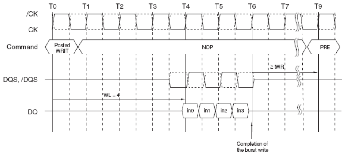
Burst Write Followed by Precharge ( WL = (RL-1) = 4 )
