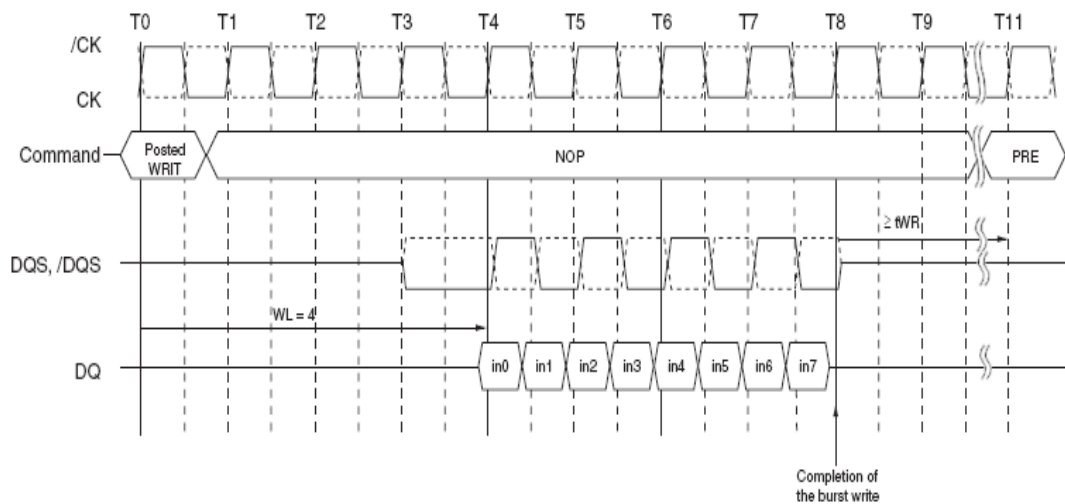
Burst Write Followed by Precharge (WL = (RL-1) = 4, BL= 8)
