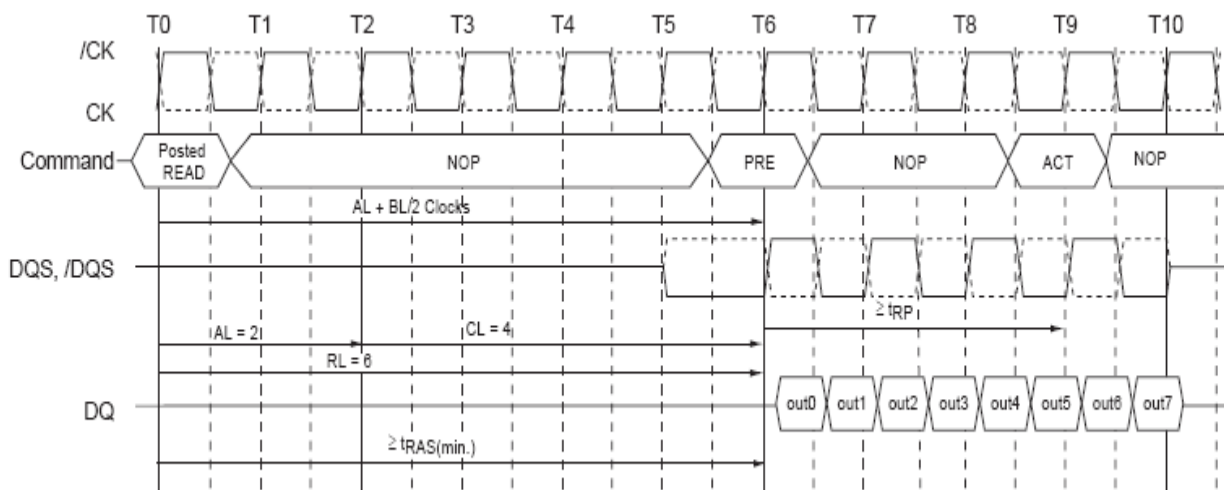
Burst Read Operation Followed by Precharge (RL = 6 (AL=2, CL=4, BL=8))
