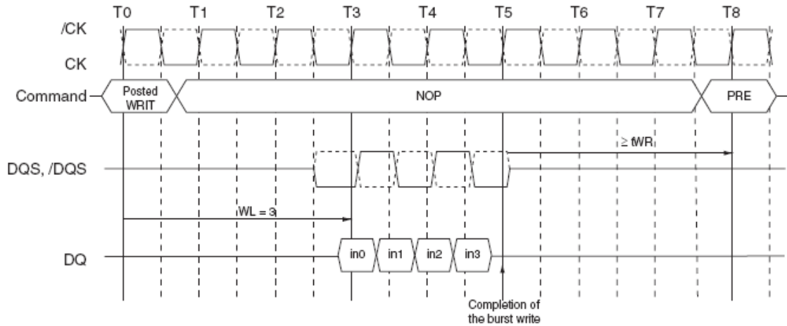
Burst Write Followed by Precharge ( WL = (RL-1) = 3 )
