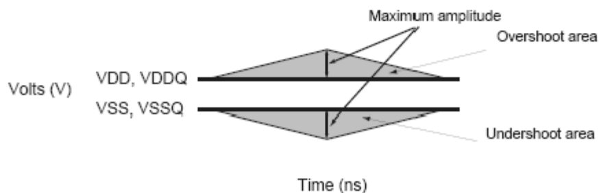
Overshoot/Undershoot Definition
