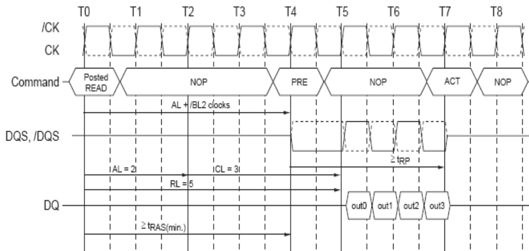
Burst Read Operation Followed by Precharge (RL = 5, BL = 4 (AL=2, CL=3))
