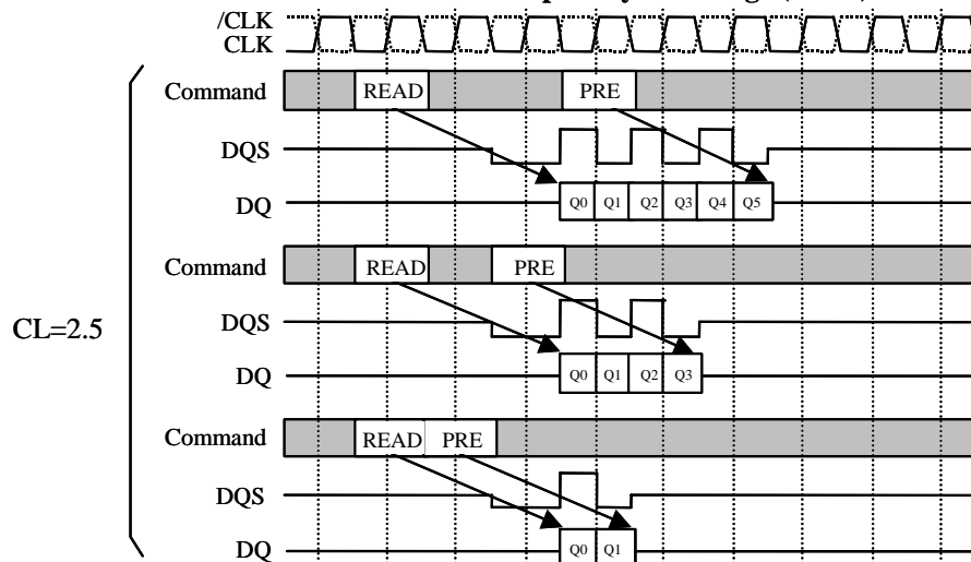
Read Interrupted by Precharge (BL=8)
