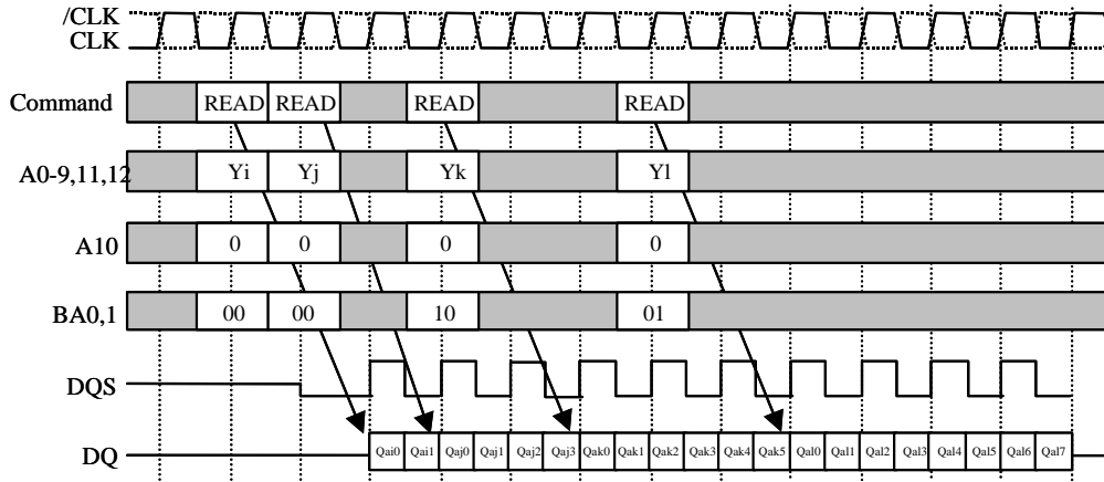
Read Interrupted by Read (BL=8, CL=2)
