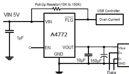
Basic Application Circuit with A4772
