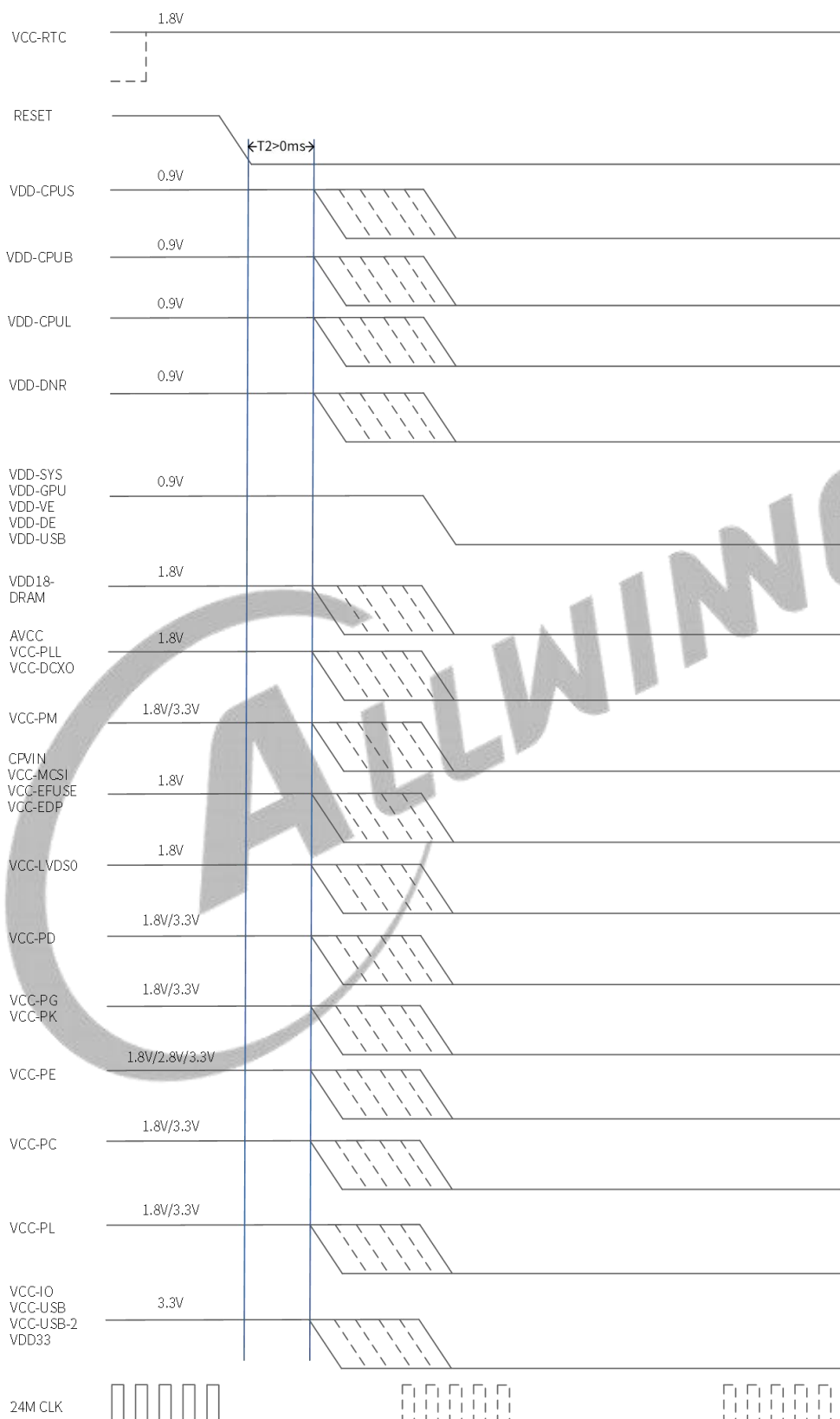
Figure 6-40 Power-off Timing
