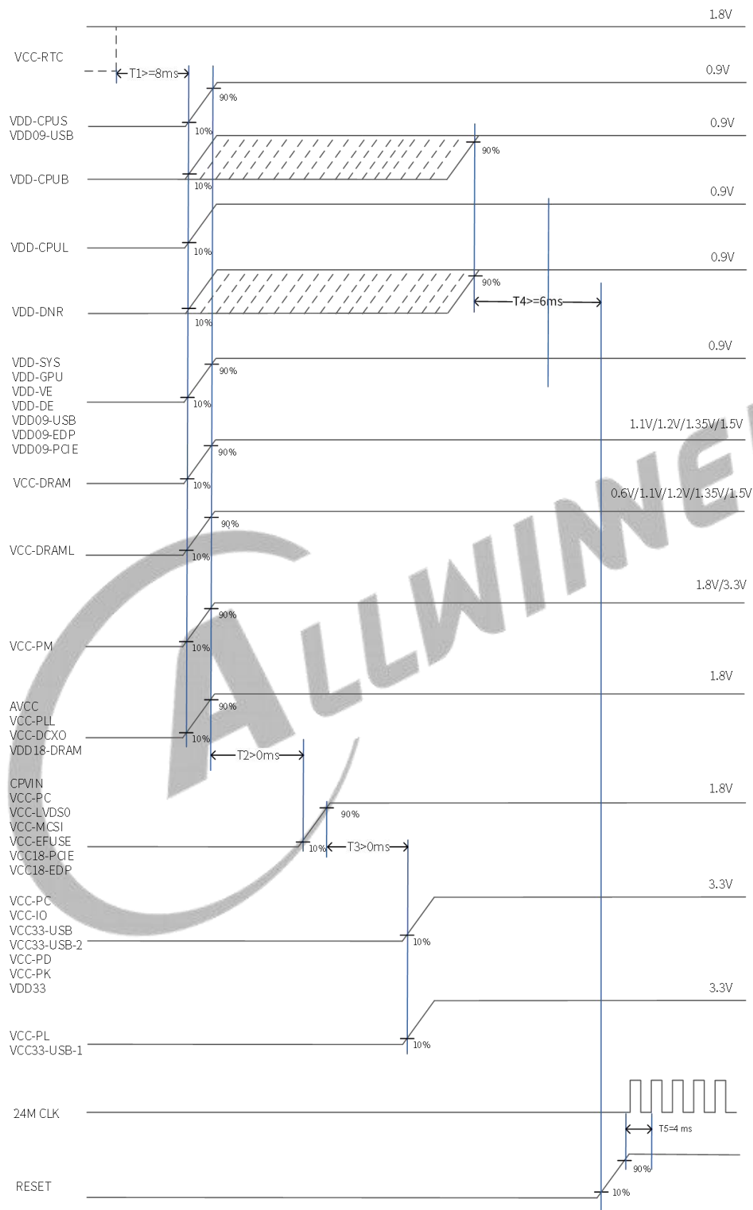
Figure 6-39 Power-on Timing
