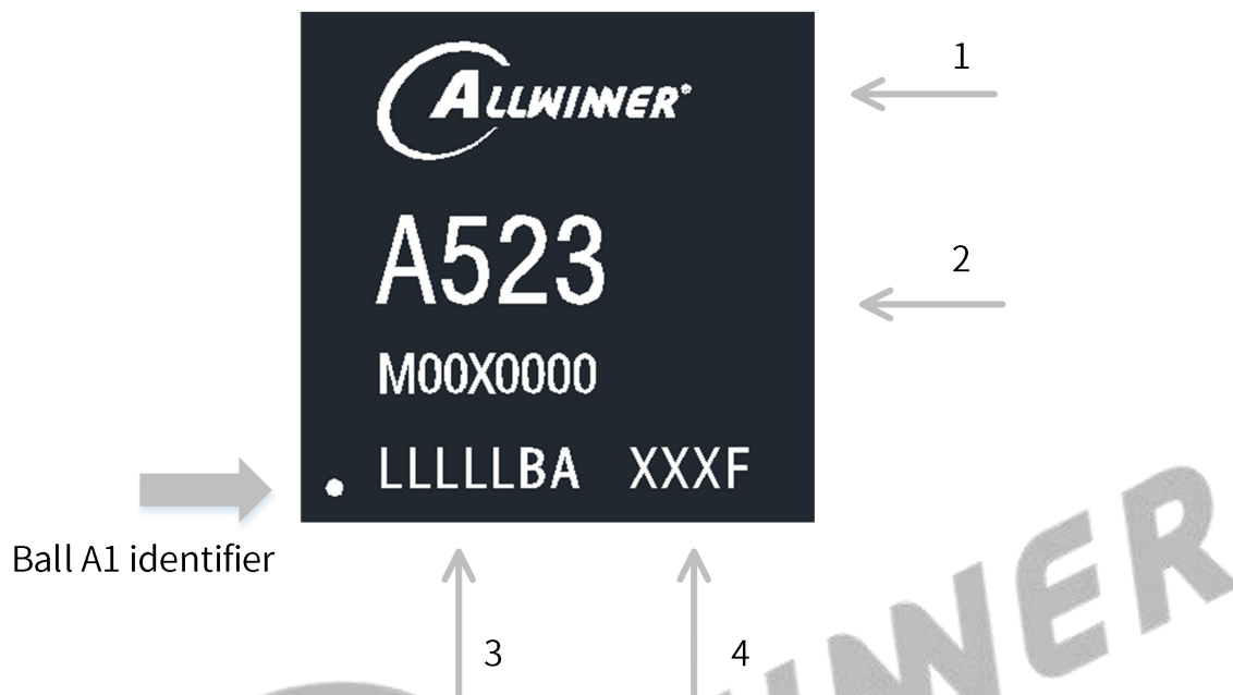
Figure 12-2 A523M00X0000 Marking
