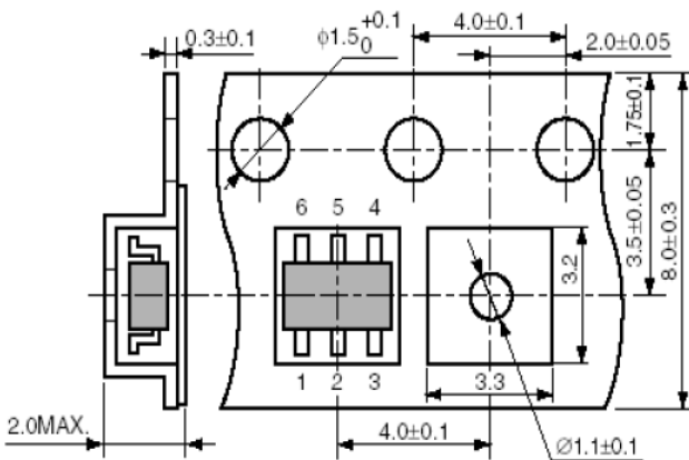
Tape Dimension
