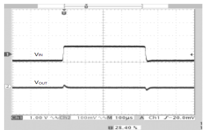
6. Line Transient Response
