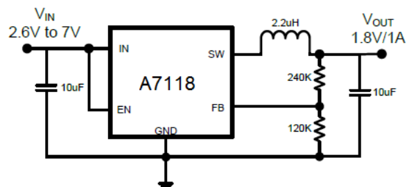
1.8V/1A Step-Down Converter
