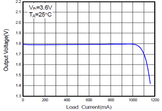
2. Output Voltage vs. Load Current
