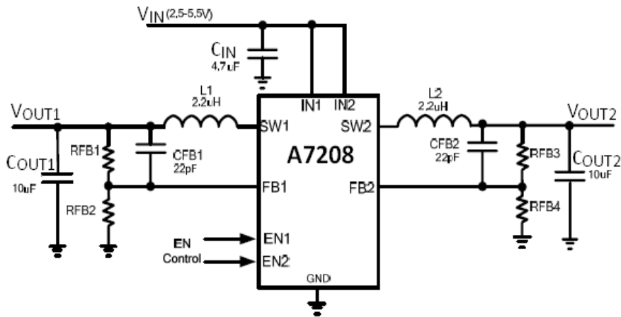
Figure 1. A7208-ADJ Typical Application
