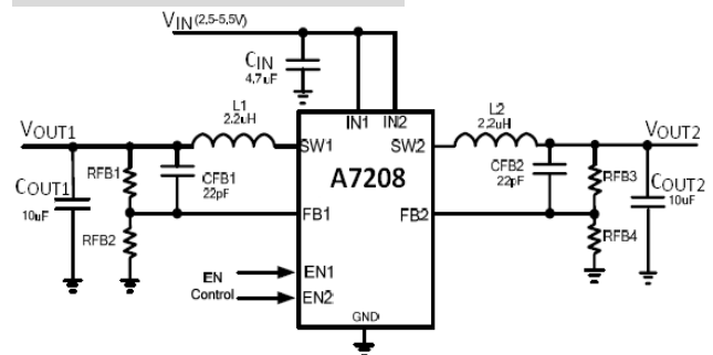
A7208-ADJ (Adjustable Type)
