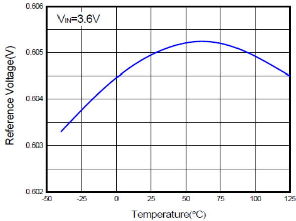
3. Reference Voltage vs. Temperature
