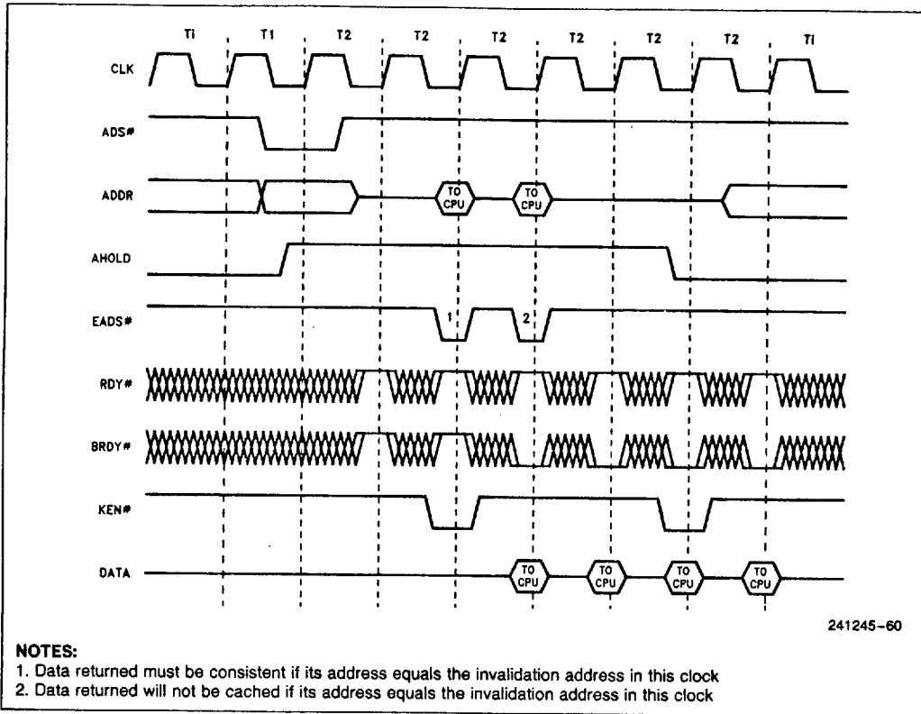
Figure 7.25. Cache Invalidation Cycle Concurrent with Line Fill
