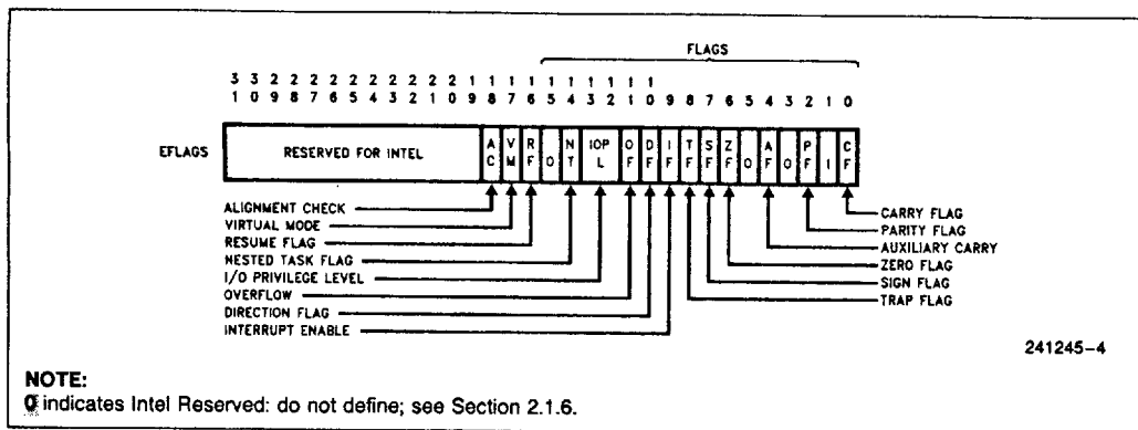
Figure 2.2. Flags Register
