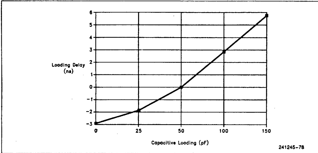
14.4.3.a TYPICAL LOADING DELAY VERSUS CAPACITIVE LOADING UNDER WORST-CASE CONDITIONS FOR A HIGH TO LOW TRANSITION ON THE INTEL486 DX2 CPU
