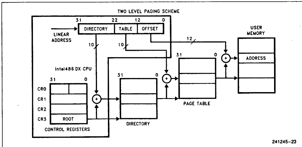
Figure 4.19. Paging Mechanism
