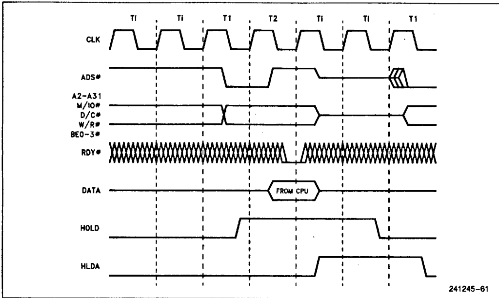
Figure 7.26a. HOLD/HLDA Cycles
