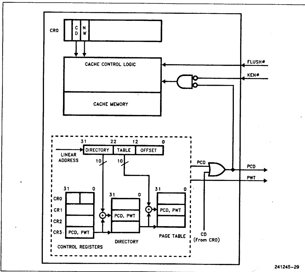
Figure 5.3. Page Cacheability
