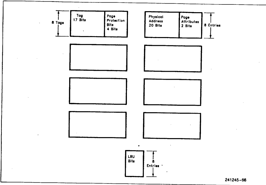
Figure 8.3. TLB Organization
