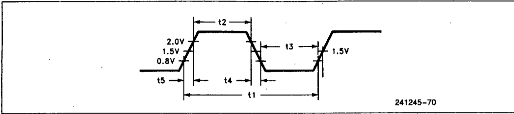
Figure 14.1. CLK Waveforms
