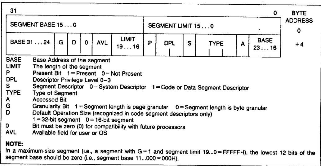
Figure 4.5. Segment Descriptors
