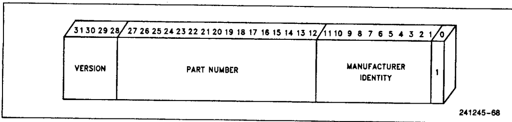
Figure 8.6. Format of Device Identification Register
