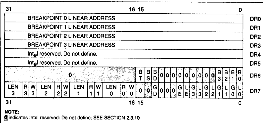
Figure 9.1. Debug Registers
