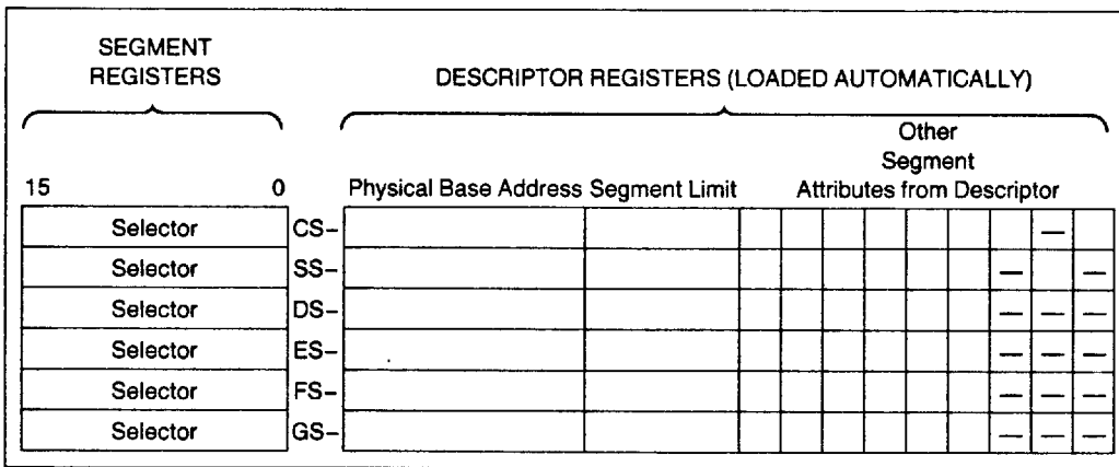
Figure 2.3. Intel486™ DX Microprocessor Segment Registers and Associated Descriptor Cache Registers
