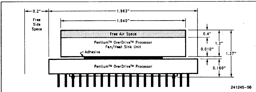
Figure 12-2. 236-Pin PGA Package with Heat Sink Attached
