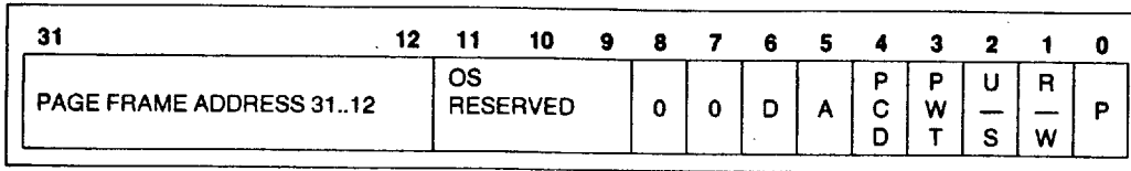
Figure 4.21. Page Table Entry (Points to Page)
