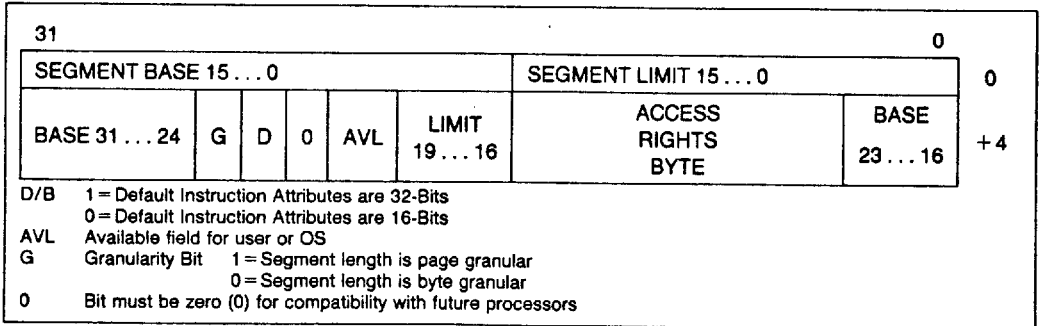
Figure 4.6. Segment Descriptors
