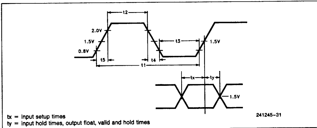
Figure 6.2. CLK waveform
