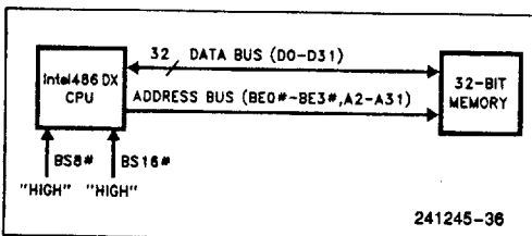
Figure 7.3. Intel486™ DX Microprocessor with 32-Bit Memory
