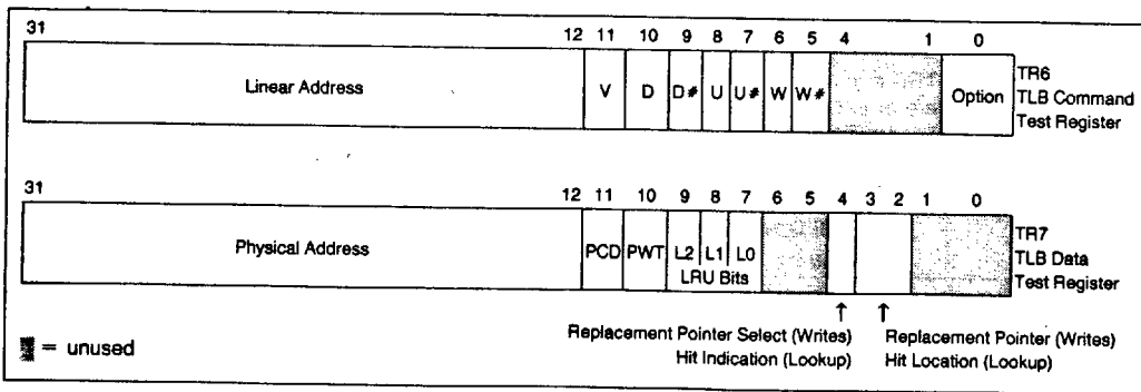
Figure 8.4. TLB Test Registers
