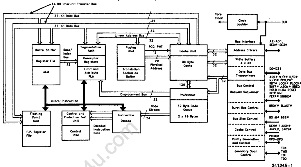
Intel486™ DX2 Microprocessor Pipelined 32-Bit Microarchitecture
