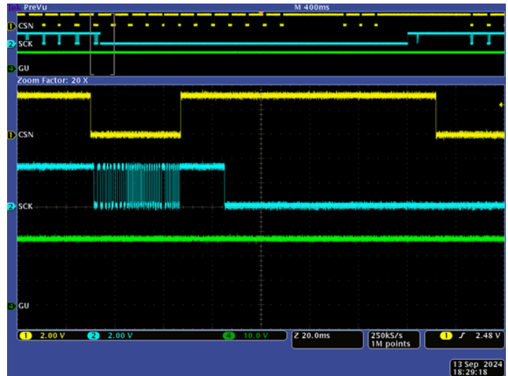
Figure 49: Short to GND Occurring When CSN is High (Zoomed-In View)
