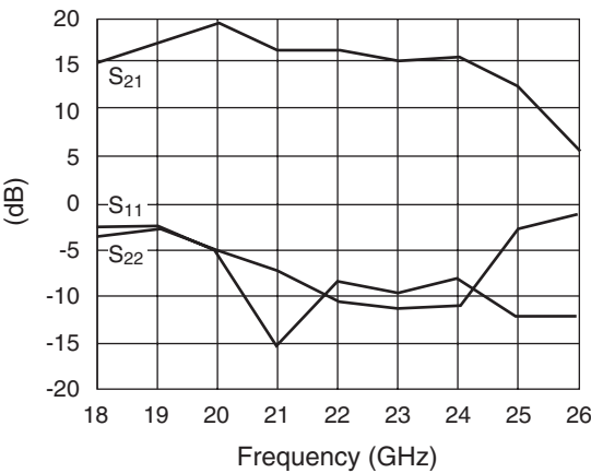
Typical Small Signal Performance S-Parameters ( V_{DS} = 6\text{ V} I_{DS} = 240\text{ mA} , T_A = 25^\circ\text{C} )
