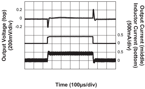
Load Transient
