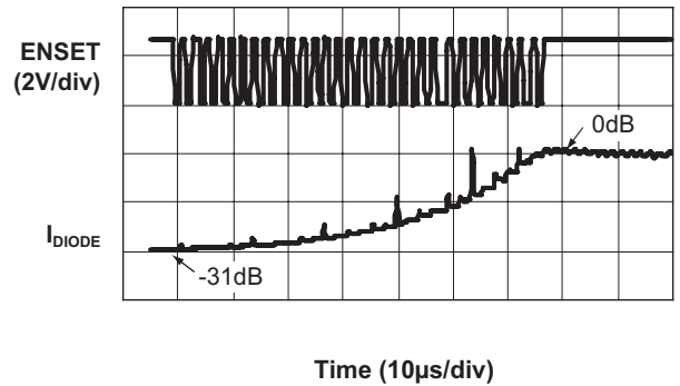
I_{DIODE} Response (-31dB to 0dB)
