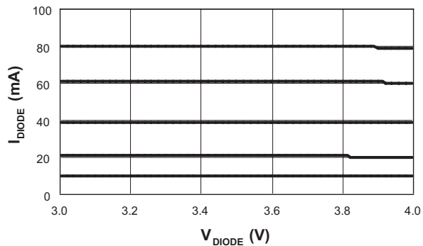
I_{DIODE} vs. V_{DIODE}
